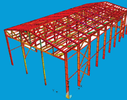
SAP2000-ANALYSIS MODEL
