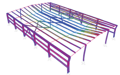
DEFLECTION ANALYSIS
