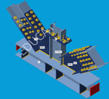
IDEA STATICA CONNECTIONS
