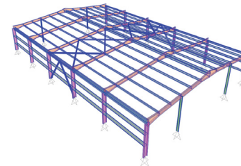
PORTAL FRAME MODEL
