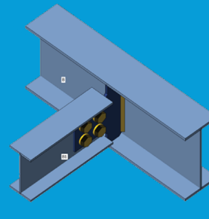
RAM CONNECTION BASE PLATES
